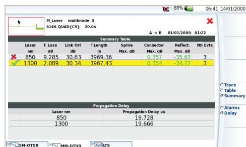
Summary & Propagation Delay table
