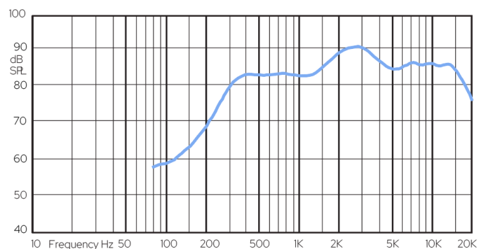
Frequency response
