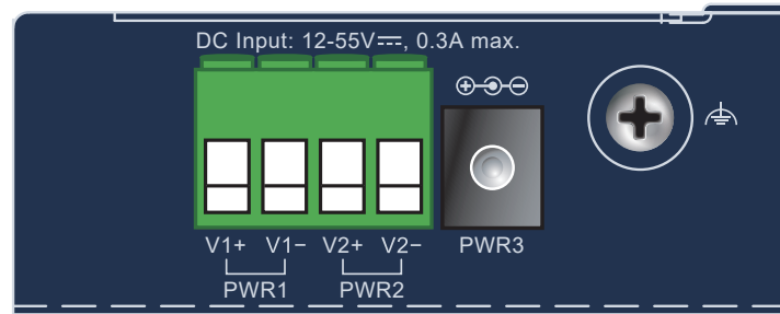
Figure 3: IGS-500T-E Top View
