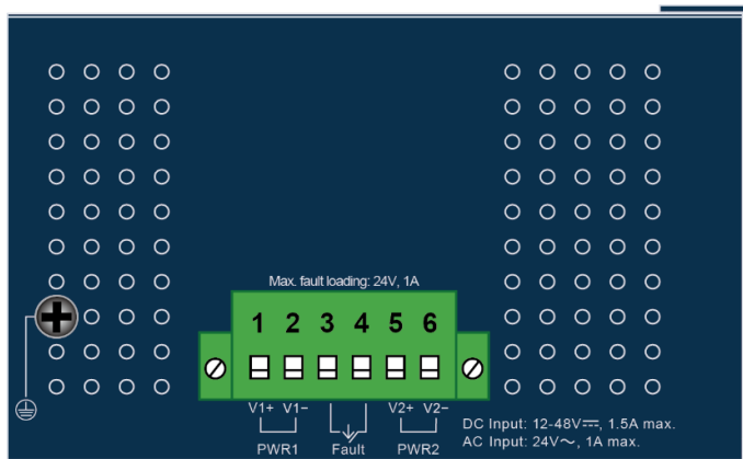
Figure 2-1-3: IGS-4215-16T2S Top View
