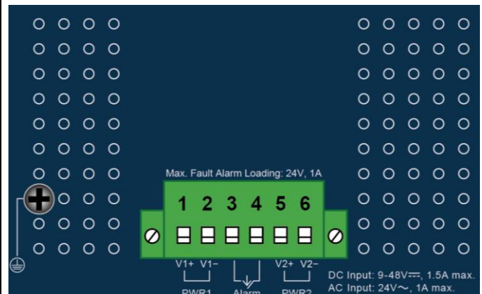
Figure 2-1-4: IGS-4215-16T2S-U Top View
