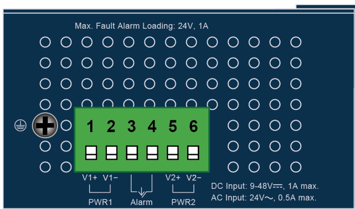
Figure 2-1-5: IGS-4215-8T2S Top View
