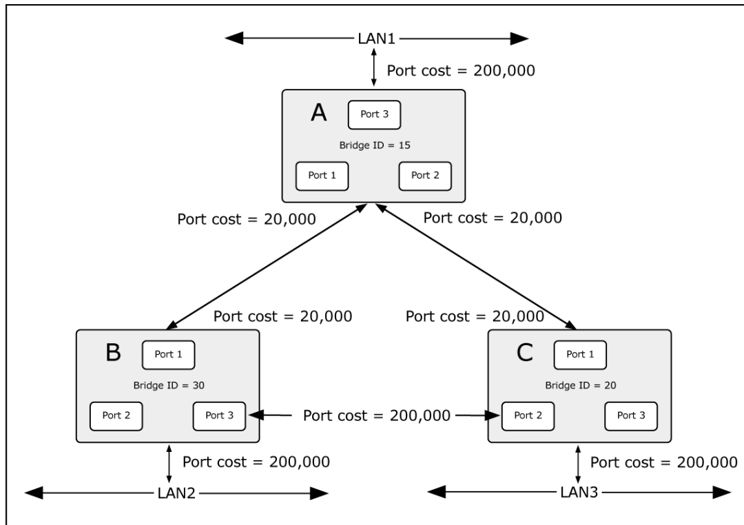
Figure 4-7-2: Before Applying the STA Rules
