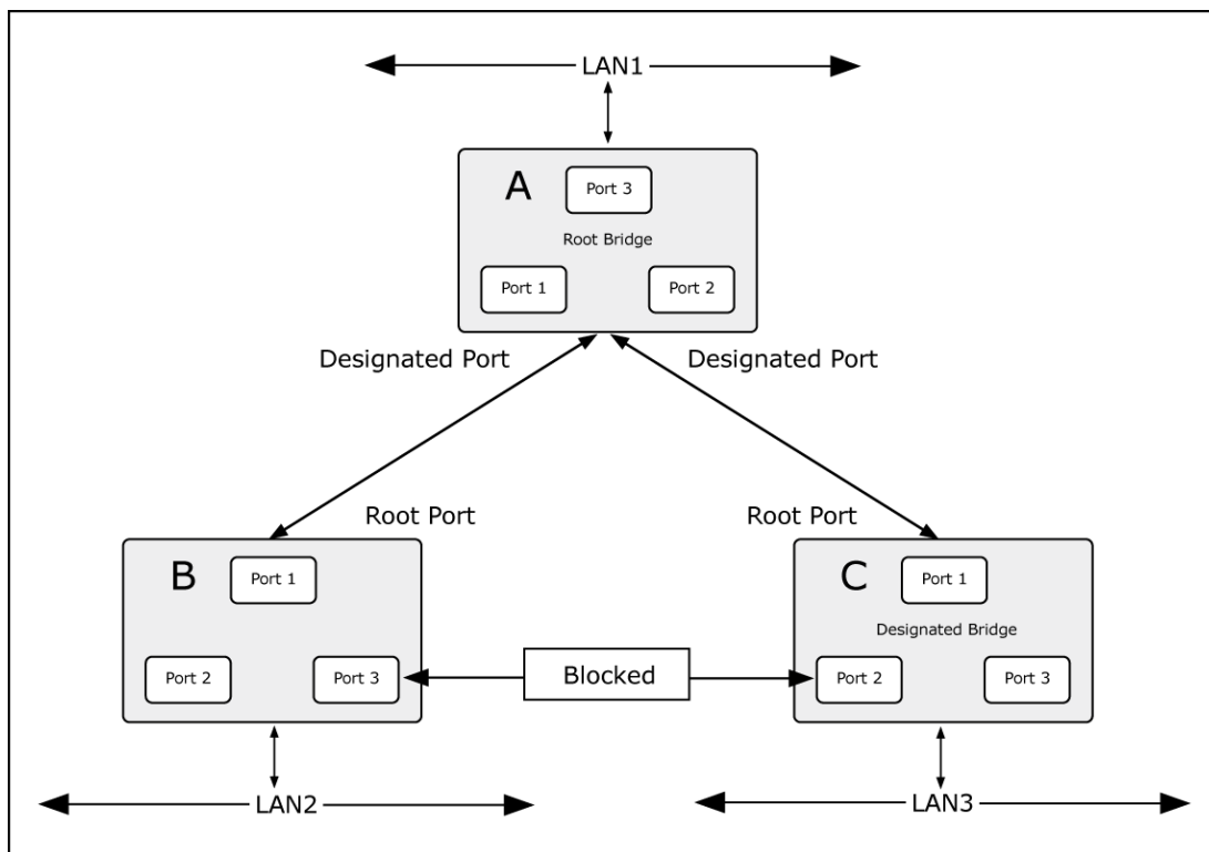
Figure 4-7-3: After Applying the STA Rules
