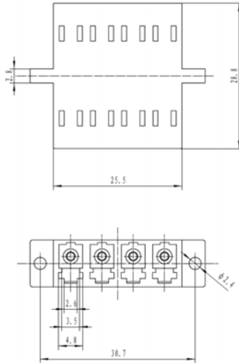
LC Quad
