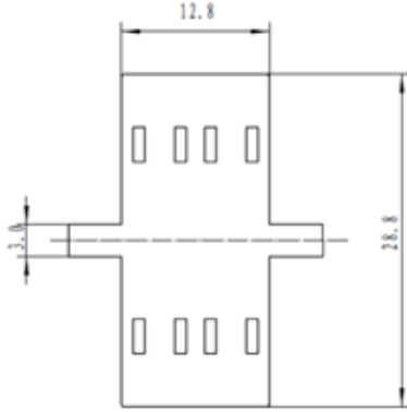
LC Duplex
