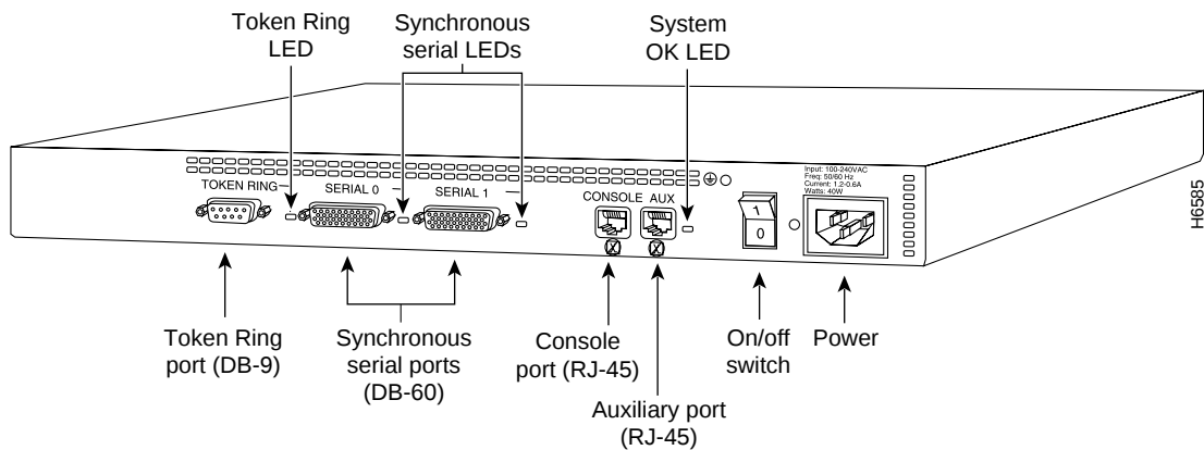
Figure 1-2 Model 2502 Router Rear Panel
