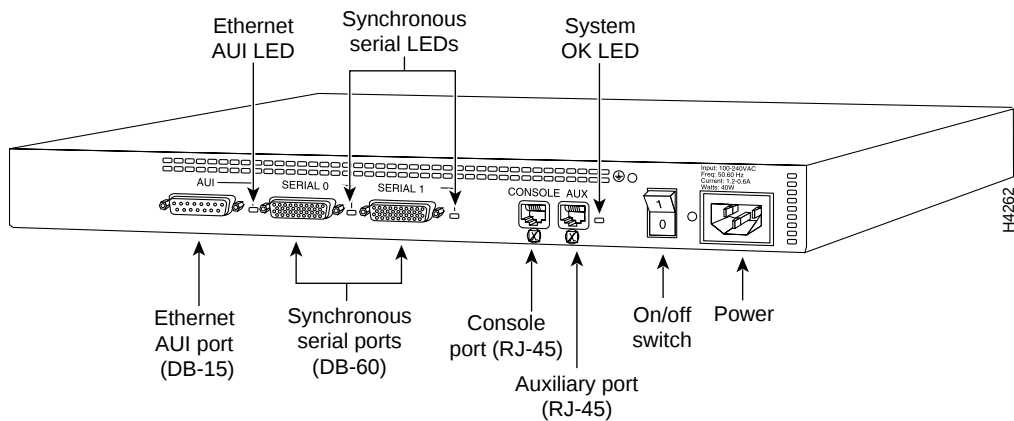
Figure 1-1 Model 2501 Router Rear Panel
