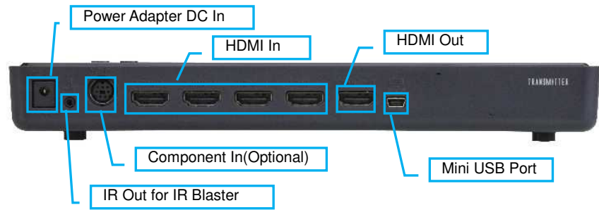
VE829T(Transmitter) Rear Panel
