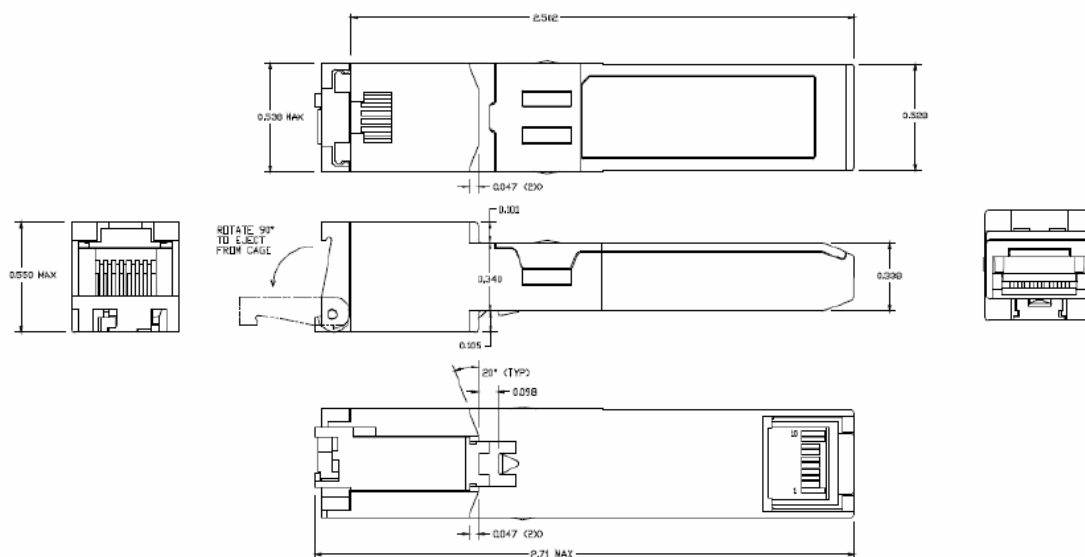
Figure 2. SFP-T mechanical dimensions
