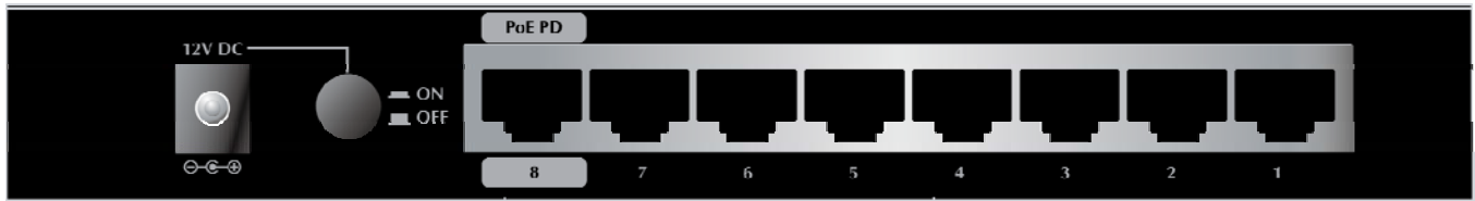
Figure 2-3 Rear panel of GSD-1002M
