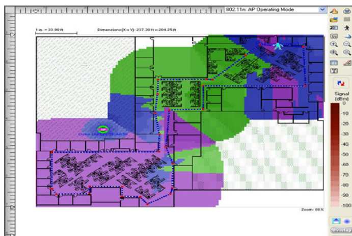
802.11n coverage maps
