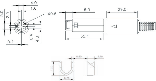
Stecker / Male
