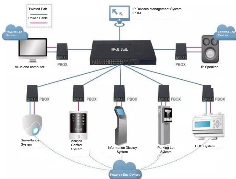
Figure 5: RG-S2910-H Powering the End Devices
