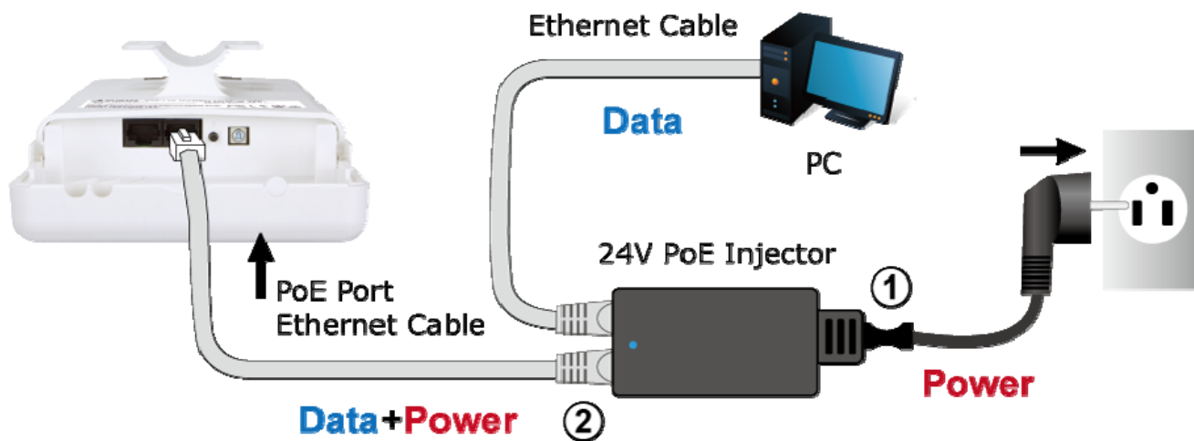
Figure 3-4 Connect the PoE injector
