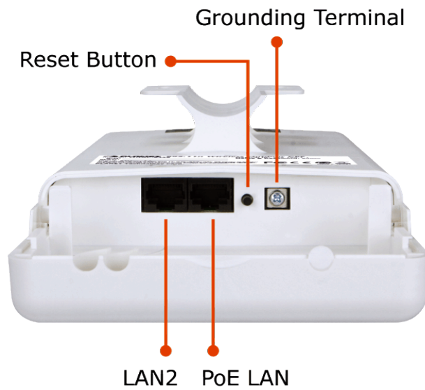
Figure 2-3 WNAP-7325 Bottom Panel
