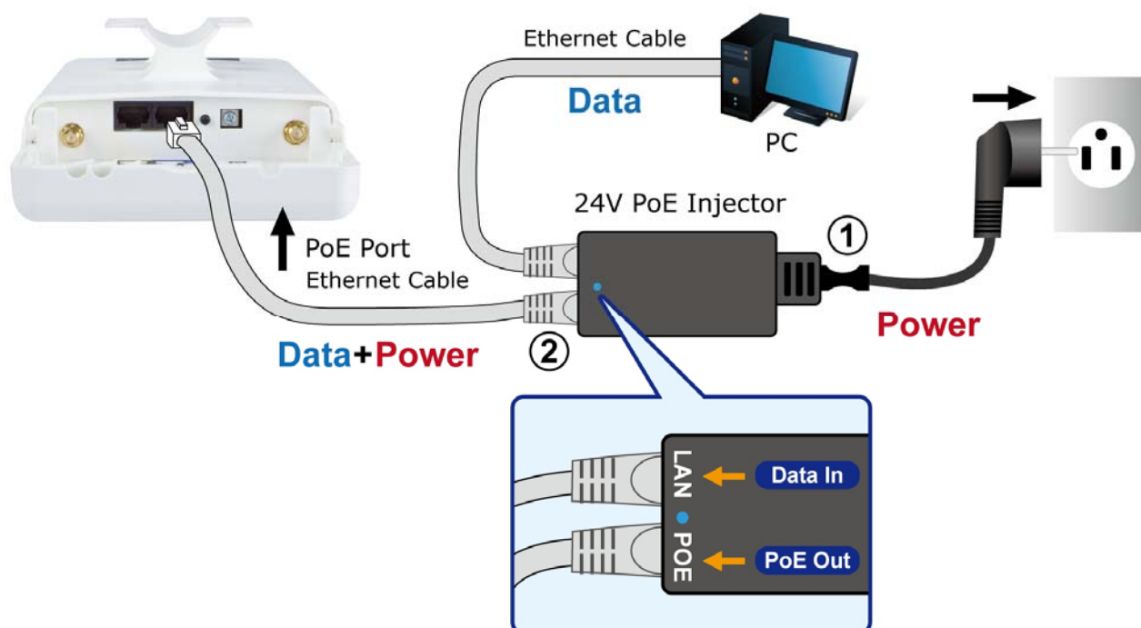
Figure 3-5 Connect the PoE injector
