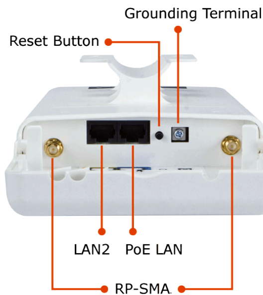
Figure 2-4 WNAP-7335 Bottom Panel
